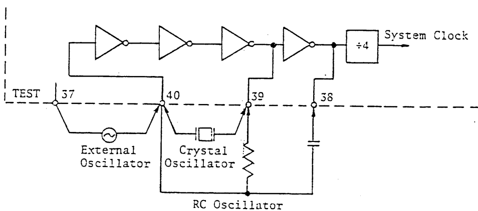
Figure 5: Clock Circuits
